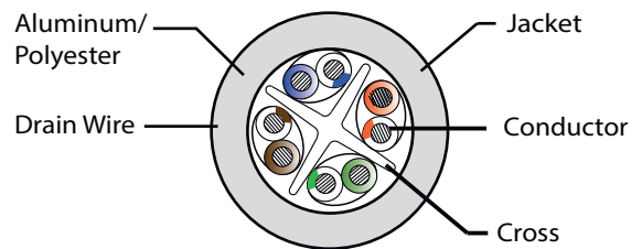
Cat 6a FTP
